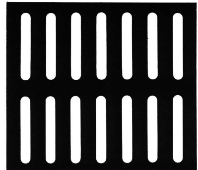
203 3×20 開孔率 32.6%
